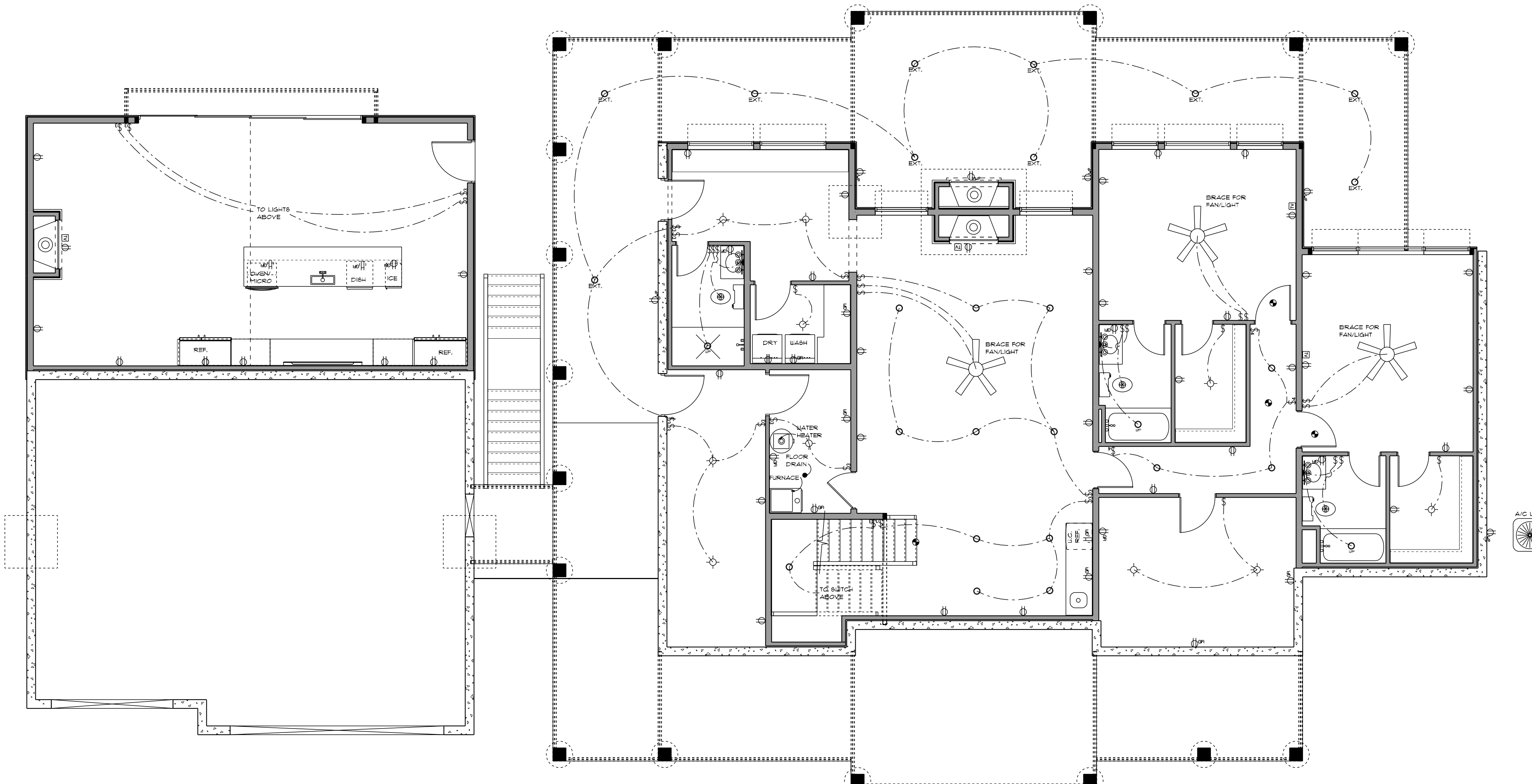
FINISHED BASEMENT ELECTRICAL PLAN SCALE 3/8" = 1'-0"
