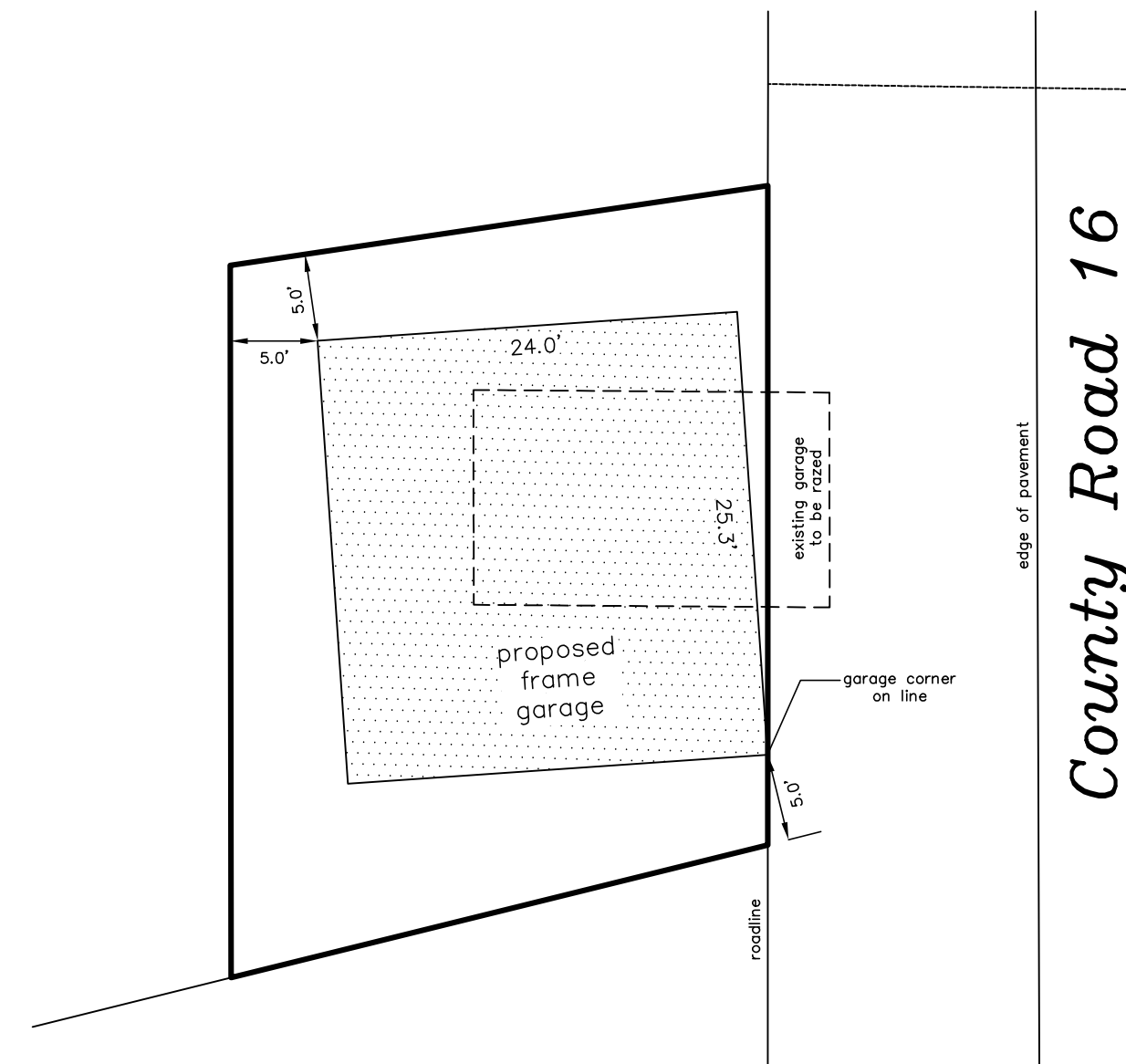
Proposed Garage Enlargement 1"=10'
