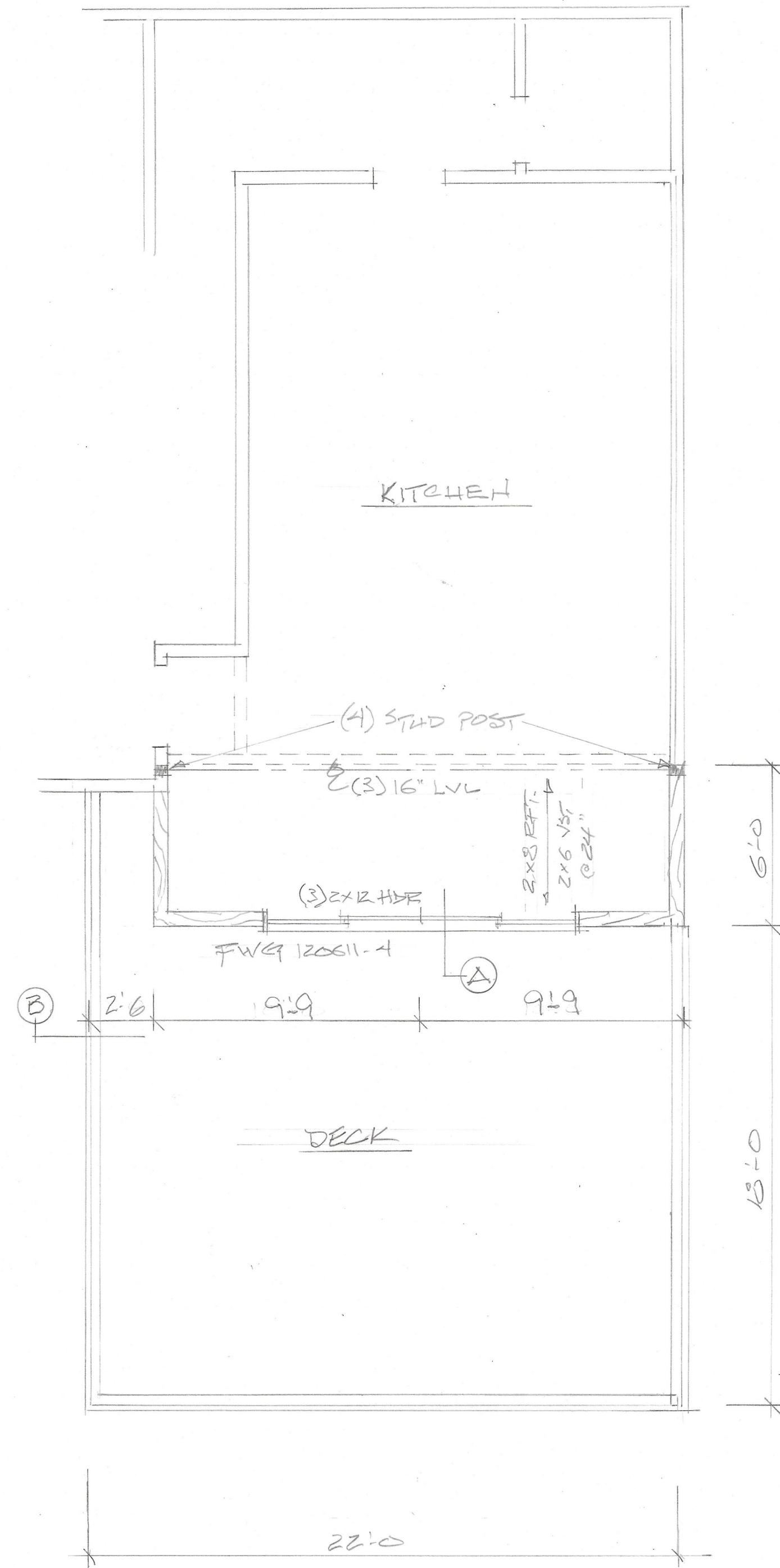
FLOOR PLAN 1/4" = 1'-0"
