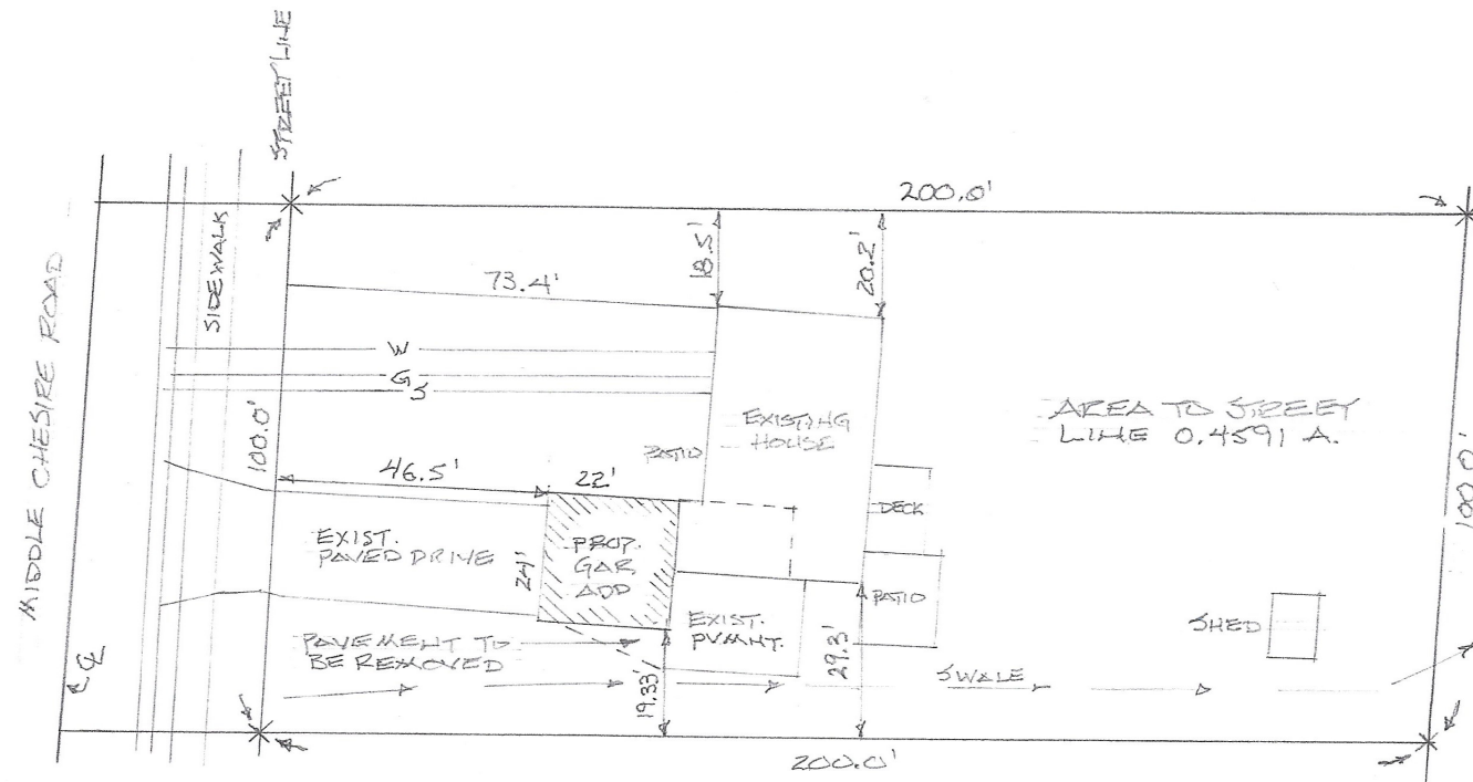
SITE PLAN 1" = 30'
