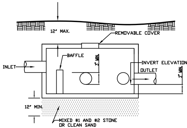
DISTRIBUTION BOX DETAILS NOT TO SCALE
