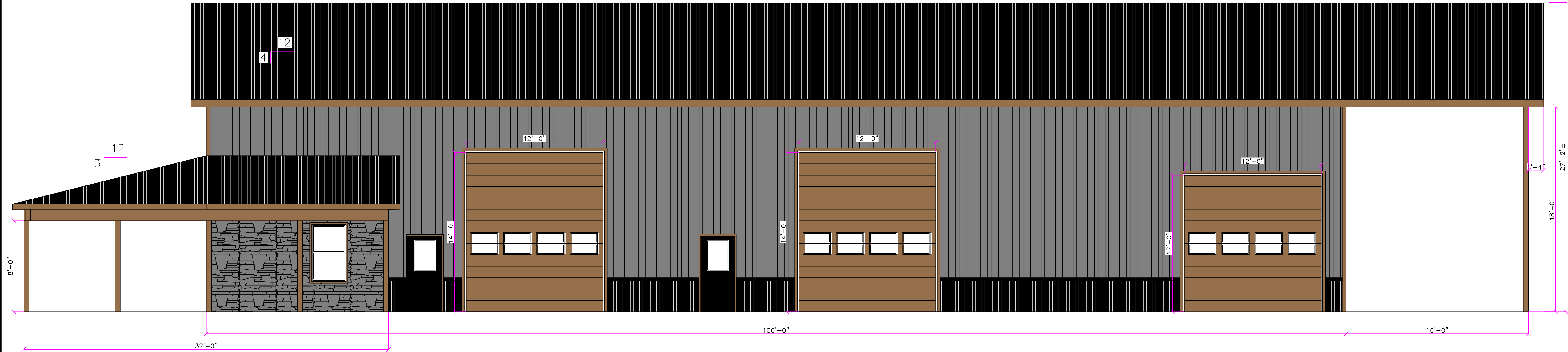
ELEVATION VIEW – SOUTH
