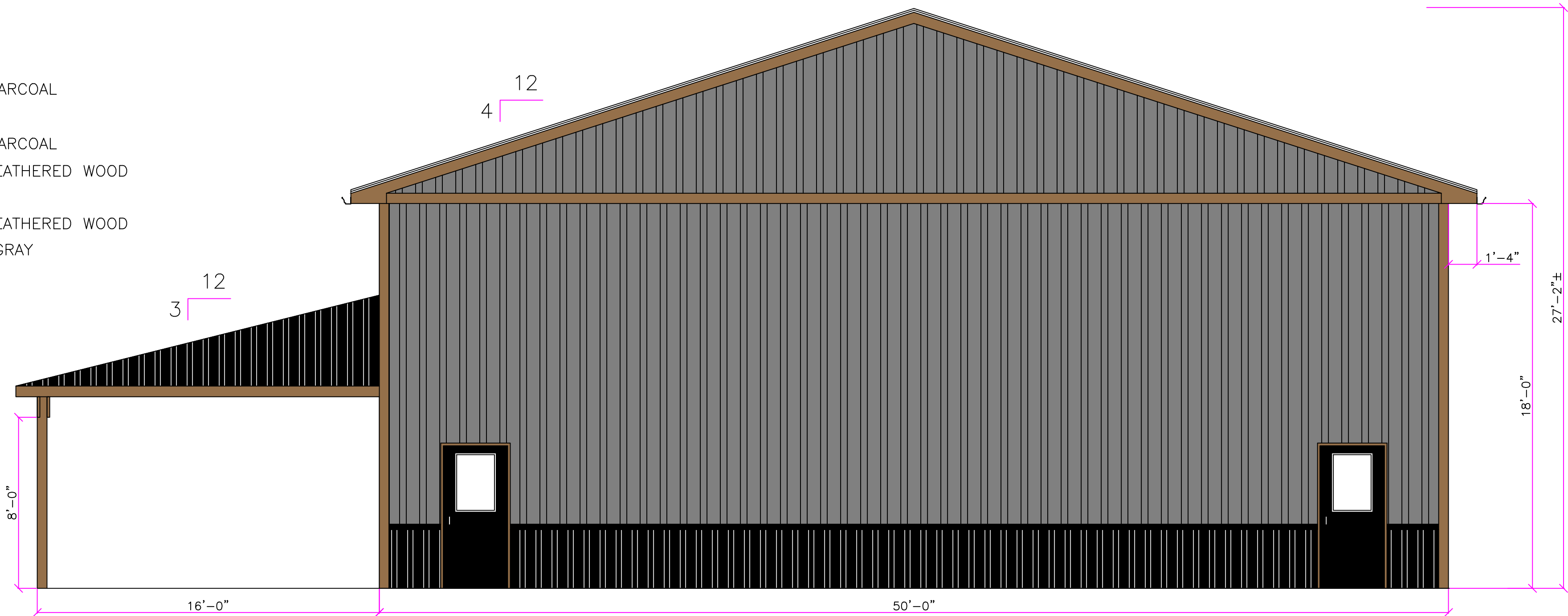
ELEVATION VIEW – EAST
