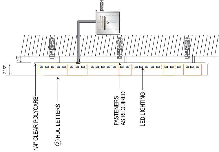
SECTION VIEW
