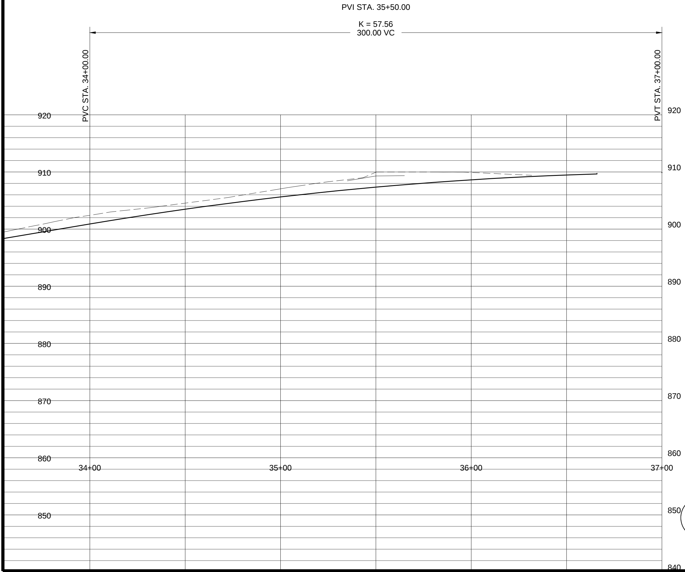
2 ROAD PROFILE 1"=30' HORIZ 1"=10' VERT
