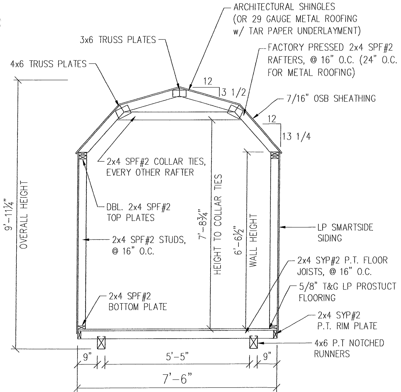
BUILDING SECTION
